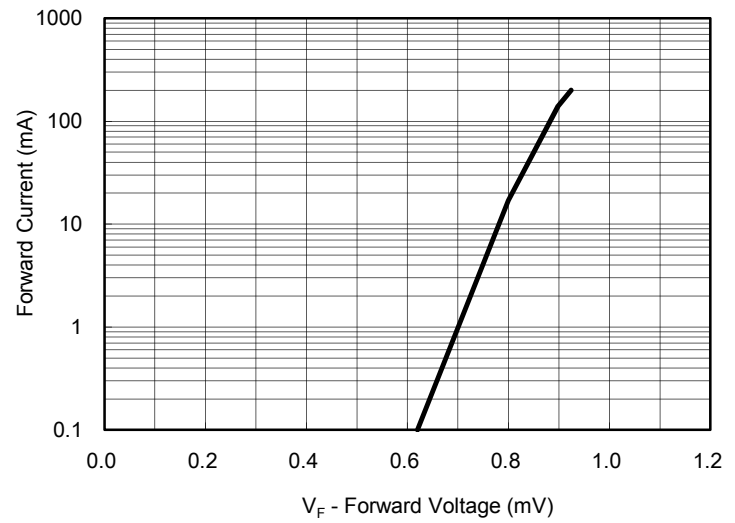
Fig. 4 Forward Current VS. Forward Voltage
